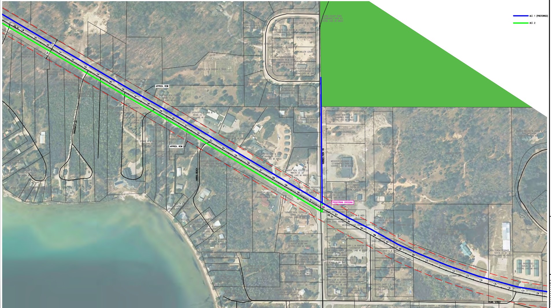
TRAIL ROUTING ALTERNATIVES: STA 134+50 - 178+50
