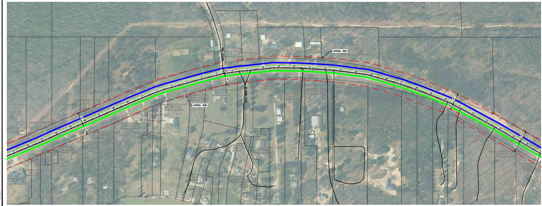
TRAIL ROUTING ALTERNATIVES: STA 101+75 - 136+00
